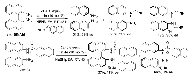
Scheme 4. Control experiments by using simple reagents.
