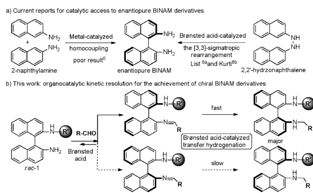
Scheme 1. General strategies for creating axially chiral BINAM derivatives.
